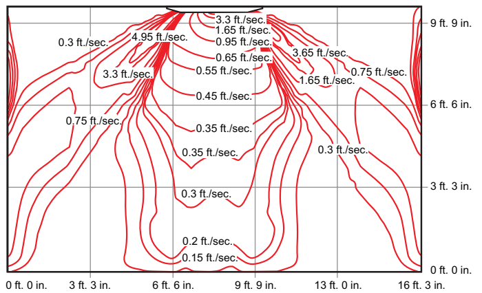
V33B015 - HEATING
