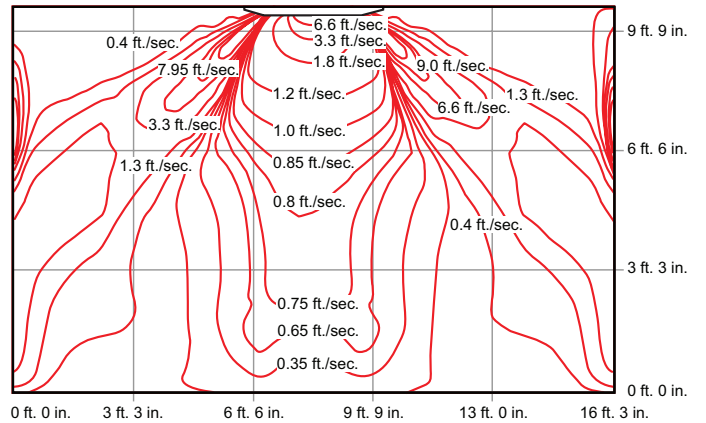
V33B048 - HEATING
