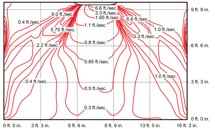
V33B036 - HEATING
