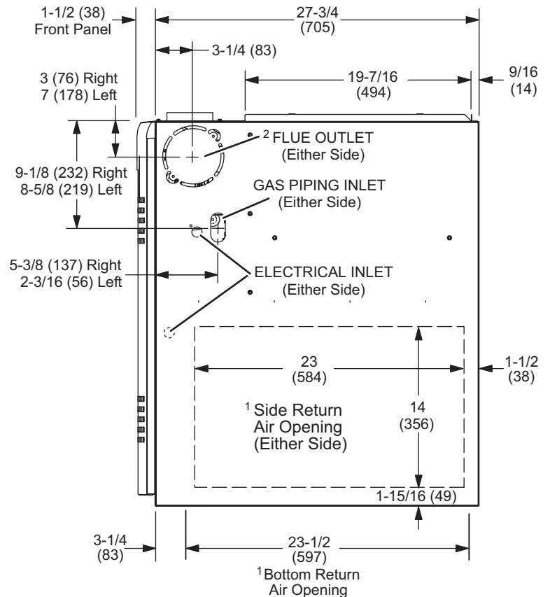
SIDE VIEW
