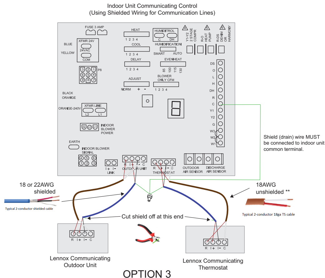
Figure 4. Lennox Communicating System Wiring Connections using Unshielded (Option 2) or Shielded Wiring (Option 3) Cabling
