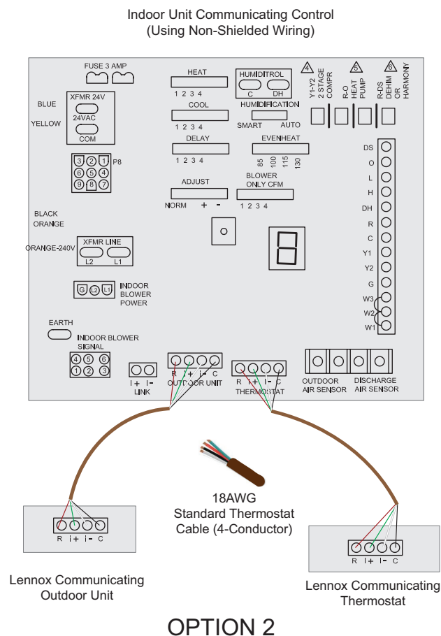
Figure 4. Lennox Communicating System Wiring Connections using Unshielded (Option 2) or Shielded Wiring (Option 3) Cabling
