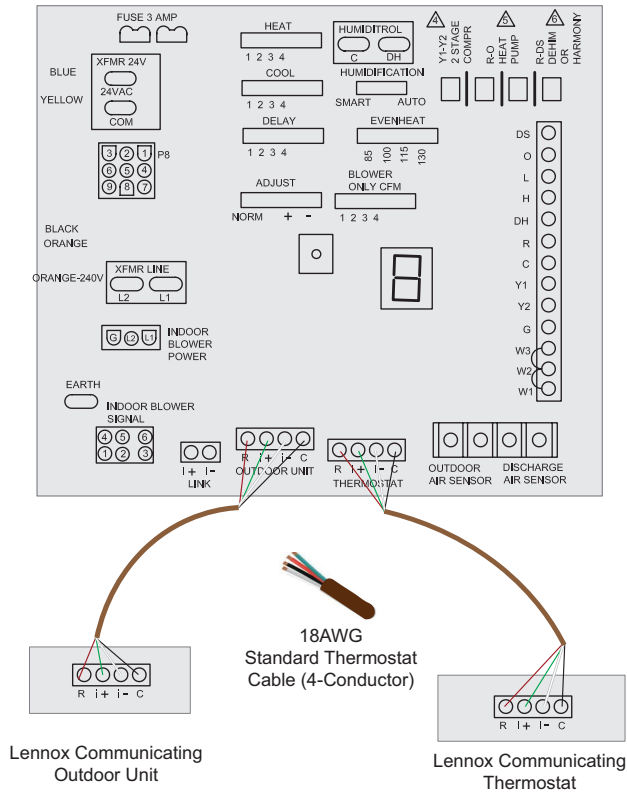
Figure 4. Lennox Communicating System Wiring Connections using Unshielded (Option 2) or Shielded Wiring (Option 3) Cabling
