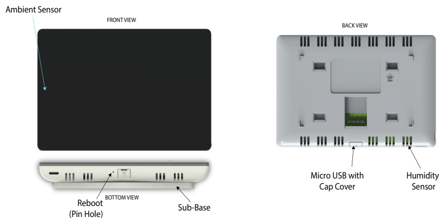
Figure 1. Thermostat External Components
