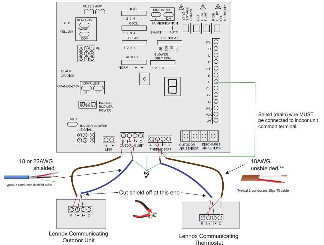
Figure 4. Lennox Communicating System Wiring Connections using Unshielded (Option 2) or Shielded Wiring (Option 3) Cabling
