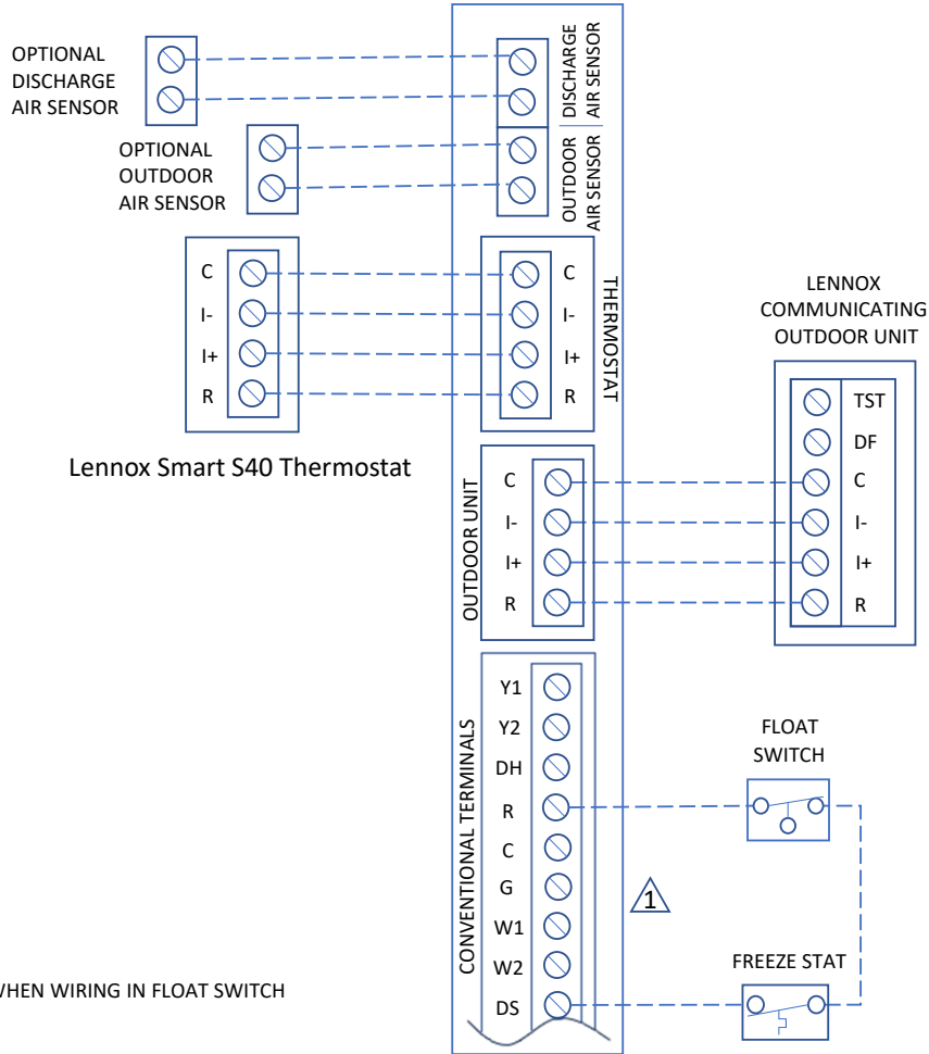
Figure 11. Lennox Smart S40 and HEPA Bypass Filter Interlock Kit and Humidifier
