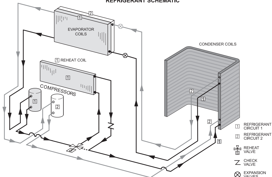
REFRIGERANT SCHEMATIC
