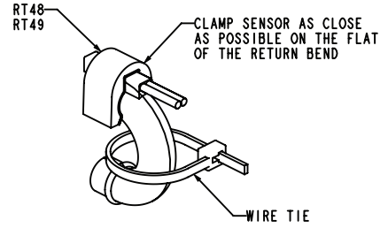
SENSOR DETAIL
