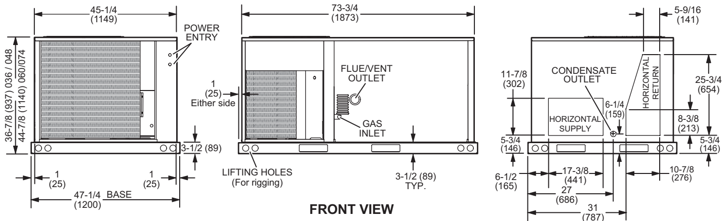
END VIEW
