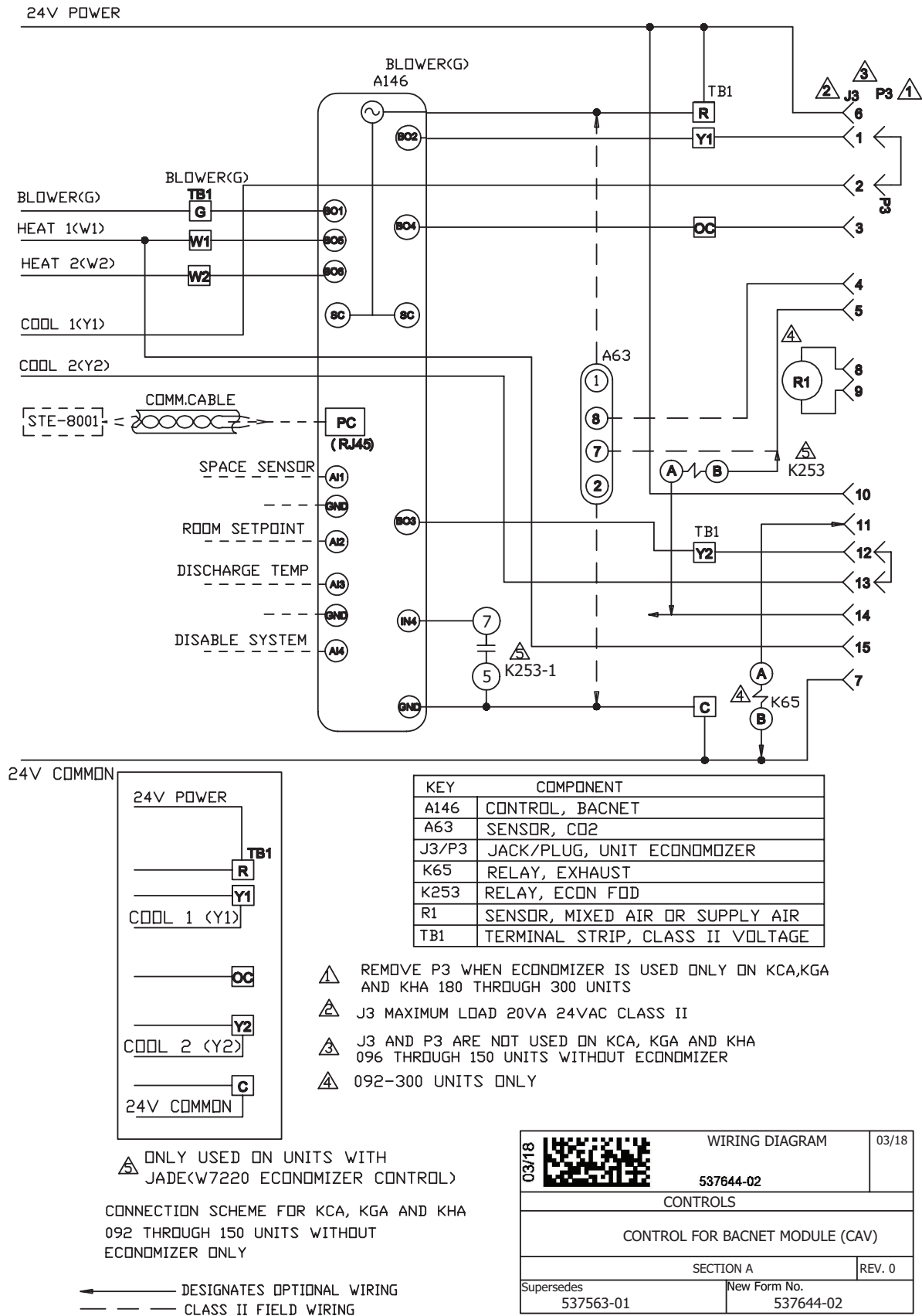
Figure 14. Control for BACnet Module KC/KG/KH A-, A+-, B- and C-Box (CAV)
