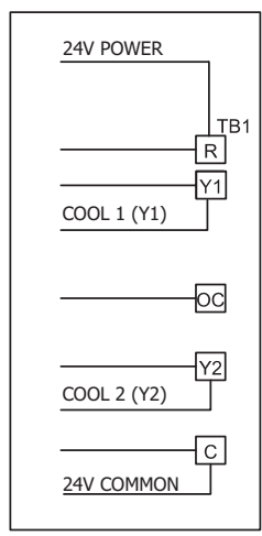
CONNECTION SCHEME FOR KDB UNITS WITHOUT ECONOMIZER ONLY
