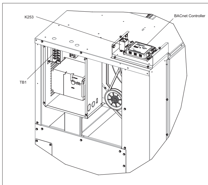
Figure 9. ELA, ELA_XA, and EL_KA Split System (Up-Flow Position Shown)
