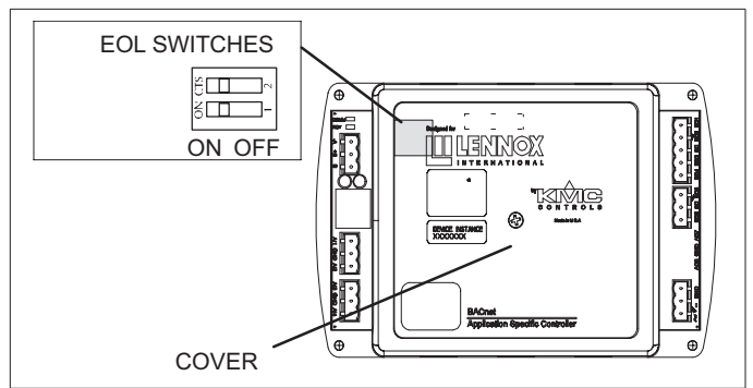
Figure 3. BACnet End-of-Line Switches (S3)
