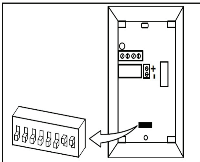
Figure 6. Wall-Mount DIP Switch Settings
