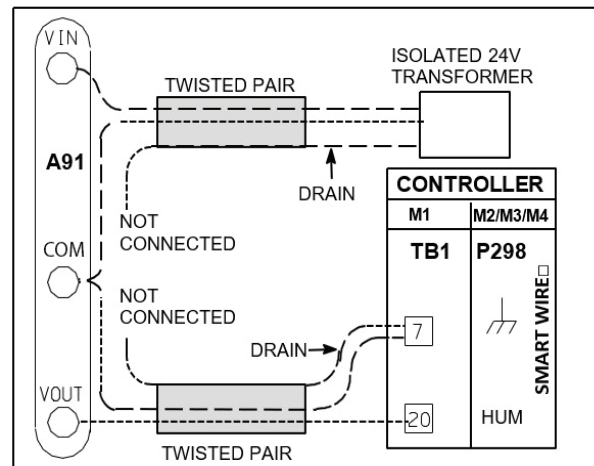
Figure 2. Field Wiring [150 ft. (46m) or Longer Runs]
