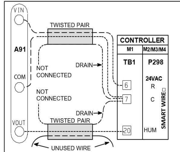
Figure 1. Field Wiring [150 ft. (46m) or Shorter Runs]
