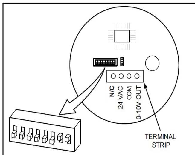
Figure 5. Duct-Mount DIP Switch Settings
