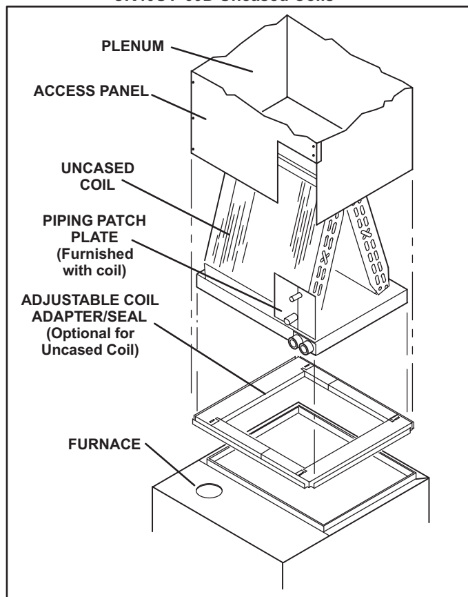
CK40UT-60D Uncased Coils
