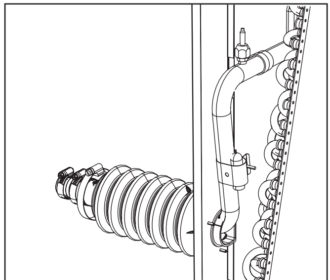
FIGURE 5. CK40UT49C-60C Suction Line with Line Set Joint Sleeve
