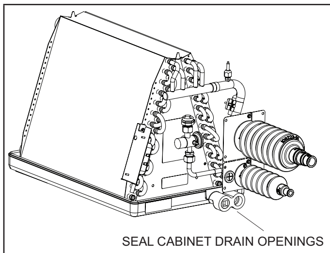
FIGURE 8. CK40UT with Line Set Joint Sleeves
