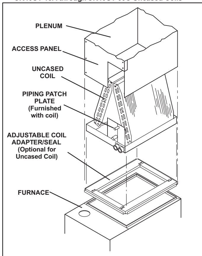
CK40UT-18A through CK40UT-60C Uncased Coils
