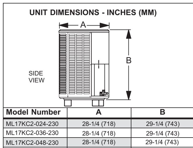
FIGURE 1. Unit Dimensions
