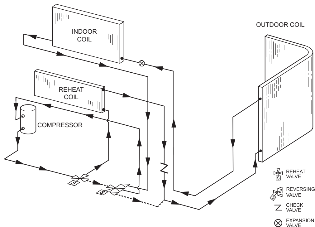
REFRIGERANT SCHEMATIC
