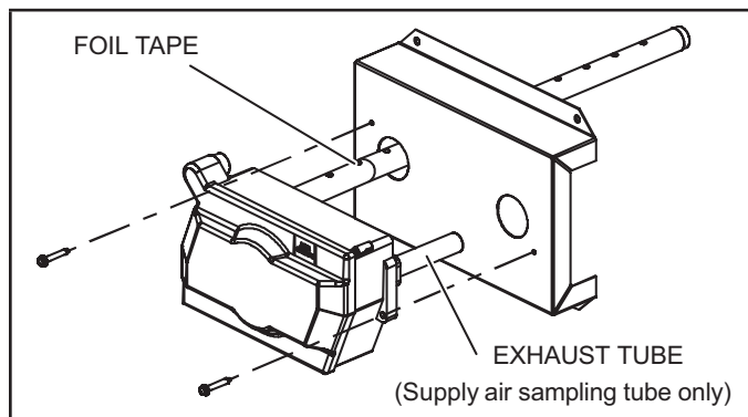
FIGURE 3 Foil tape installation
