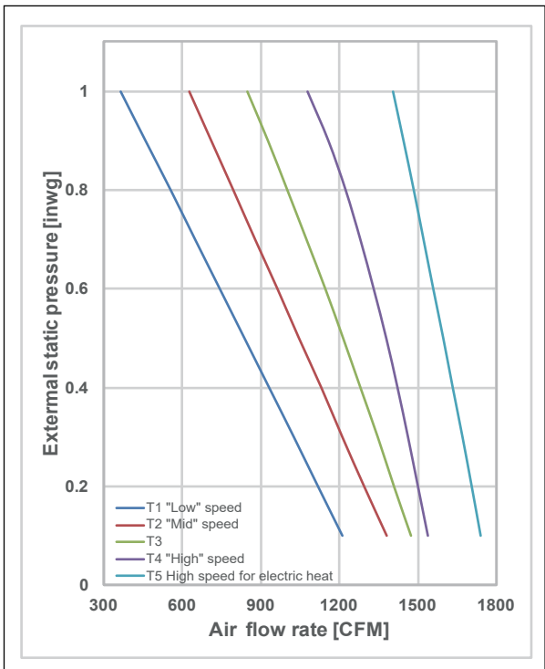
6) VVCC048S4-4P
