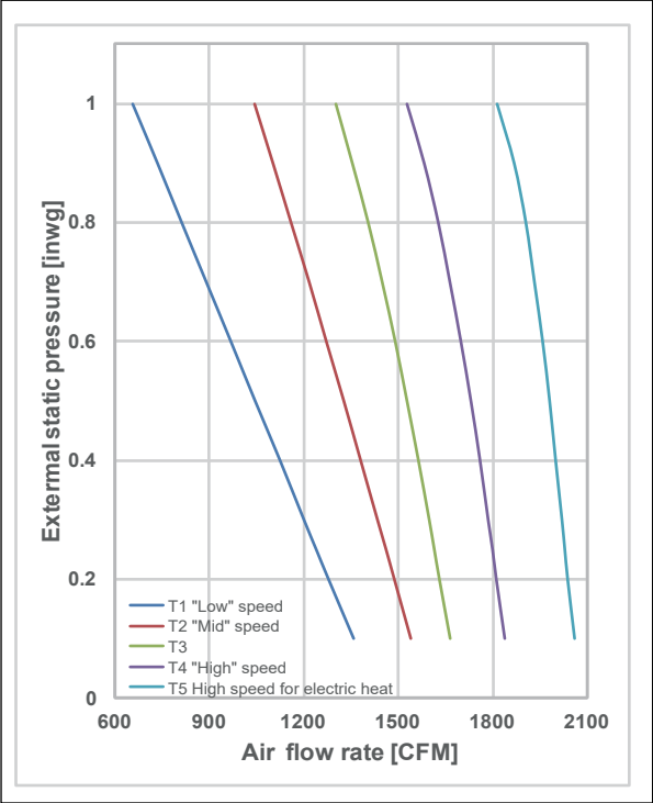
8) VVCC060S4-4P
