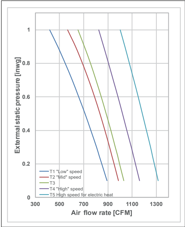
4) VVCC030S4-4P
