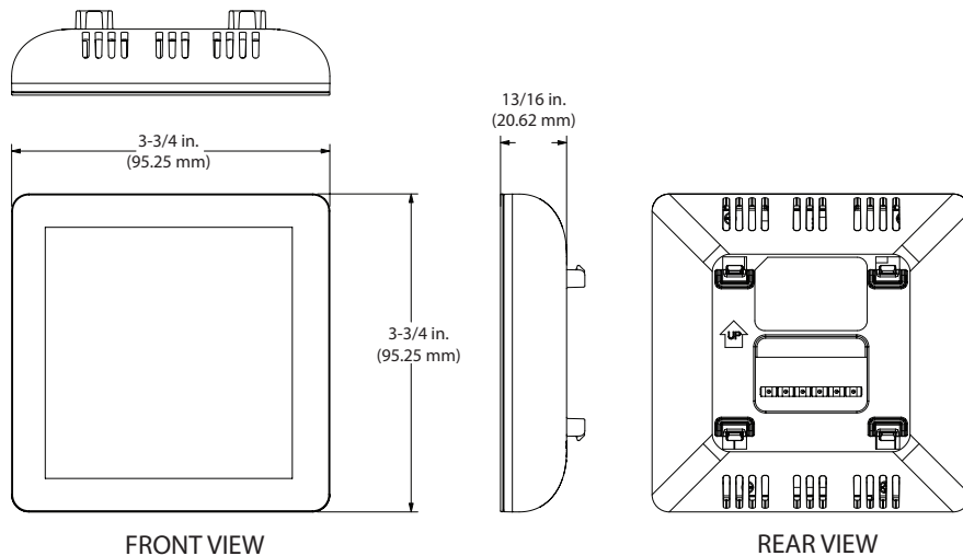
Figure 1. Thermostat Dimensions
