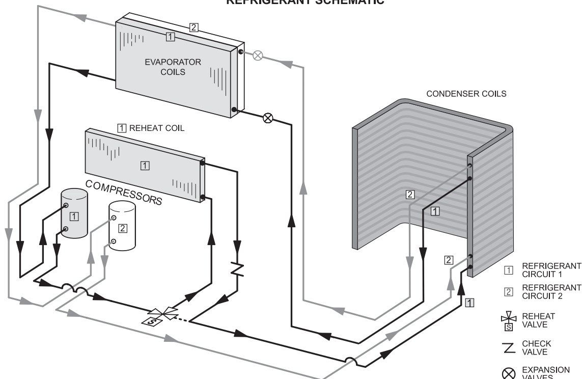
REFRIGERANT SCHEMATIC
