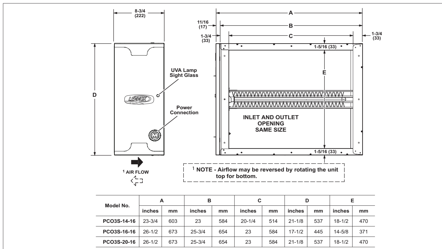
Figure 2. Dimensions
