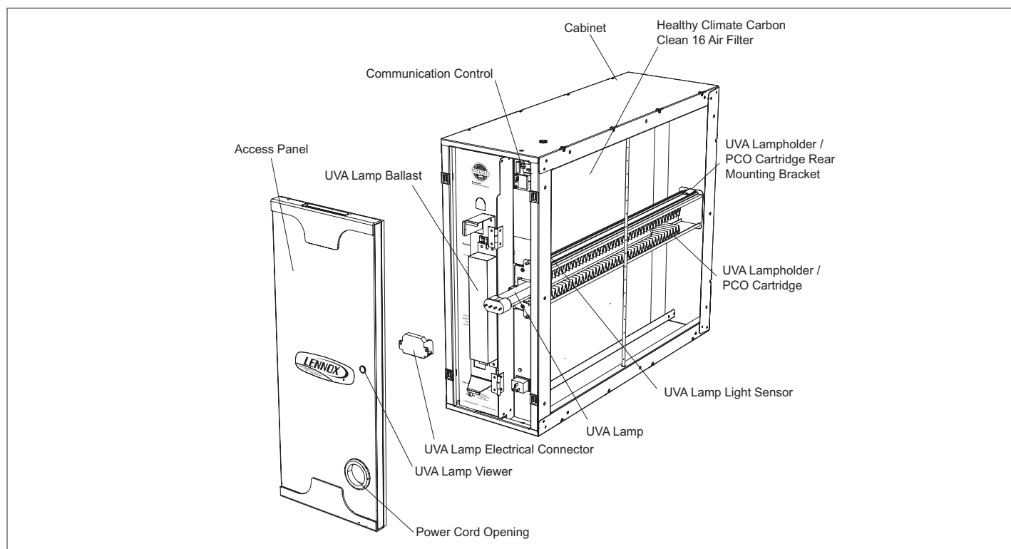
Figure 1. Parts Identification
