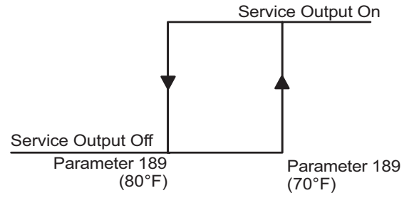
Output NOT Inverted - Input source 9 only
