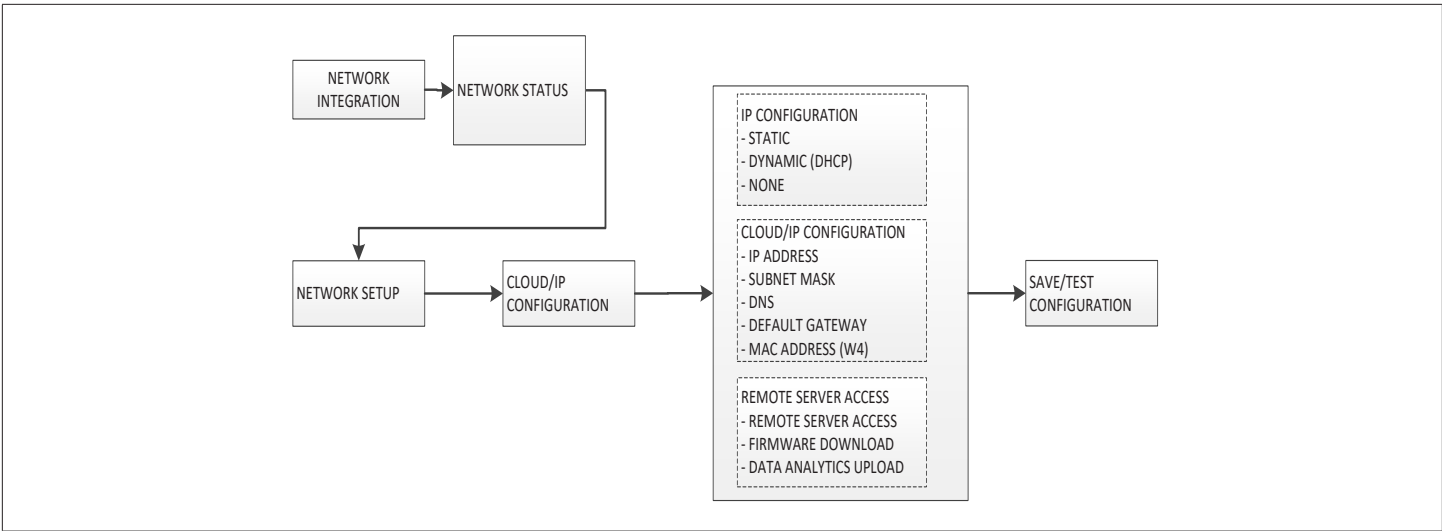
Figure 14. Cloud/IP Configuration Menu Structure
