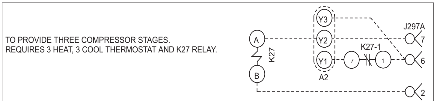
Figure 30. Third-Stage Cool (Parameter 111) Wiring
