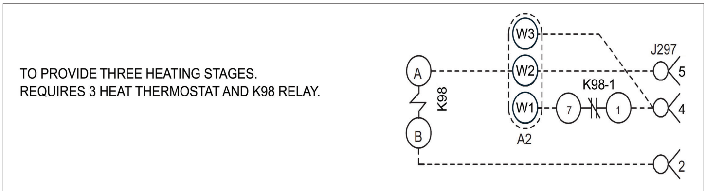
Figure 31. Third Stage Heat (Parameter 112) Wiring
