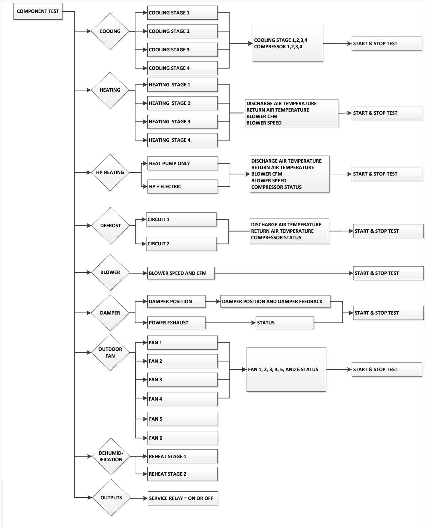
Figure 24. Component Test Menu Structure
