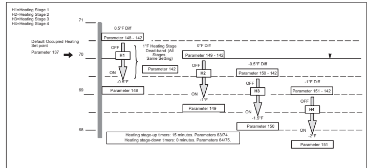
Figure 33. Room Sensor Stages for Gas / Electric Units - Heating (default values shown)
