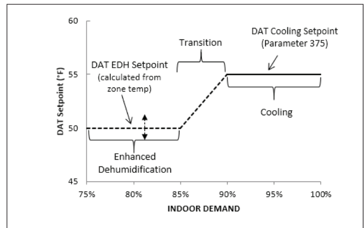
Figure 38. Modes of Operation
