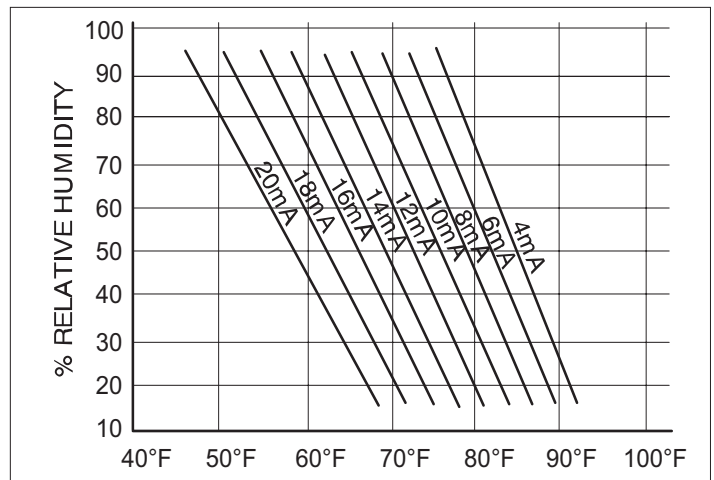
Figure 33. Enthalpy Sensor Output Current
