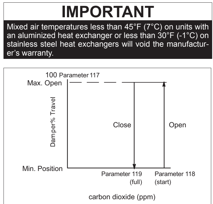
Figure 36. Set Point Control Indoor Air Quality Option
