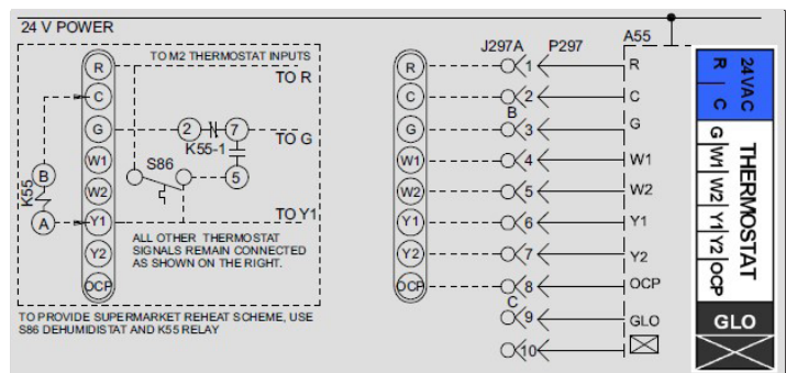
Figure 31. Supermarket Reheat Diagram
