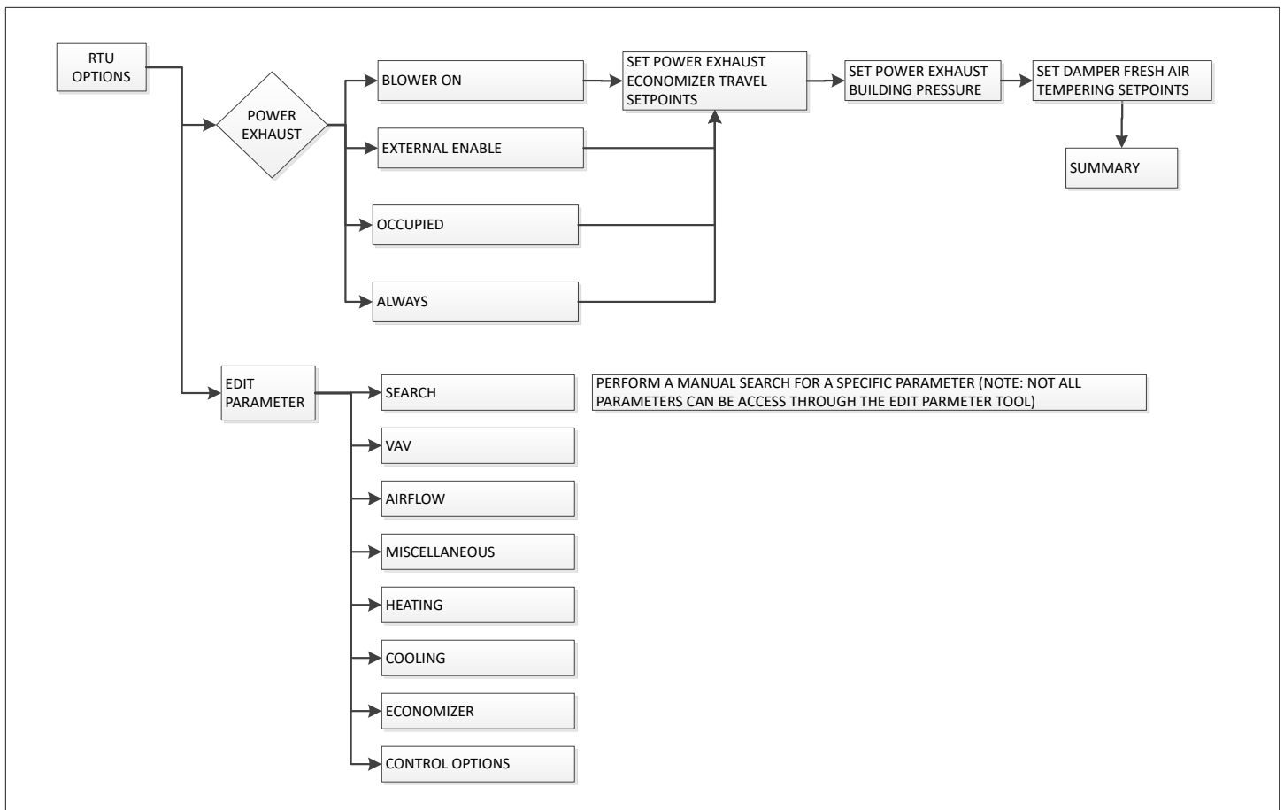
Figure 25. Settings - Power Exhaust and Edit Parameter
