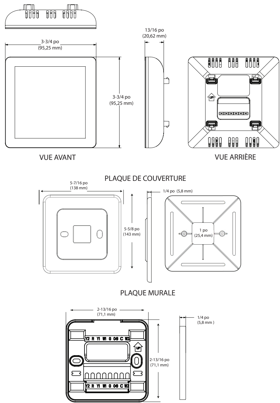
Figure 1. Thermostat intelligent M40 de Lennox, couvercle et plaque murale
