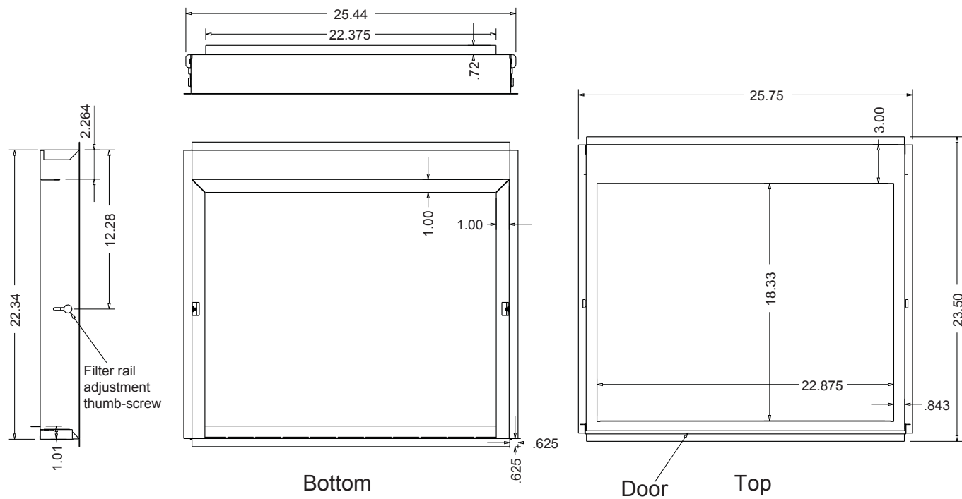
V1FBS03-4P Dimensions (inches)
