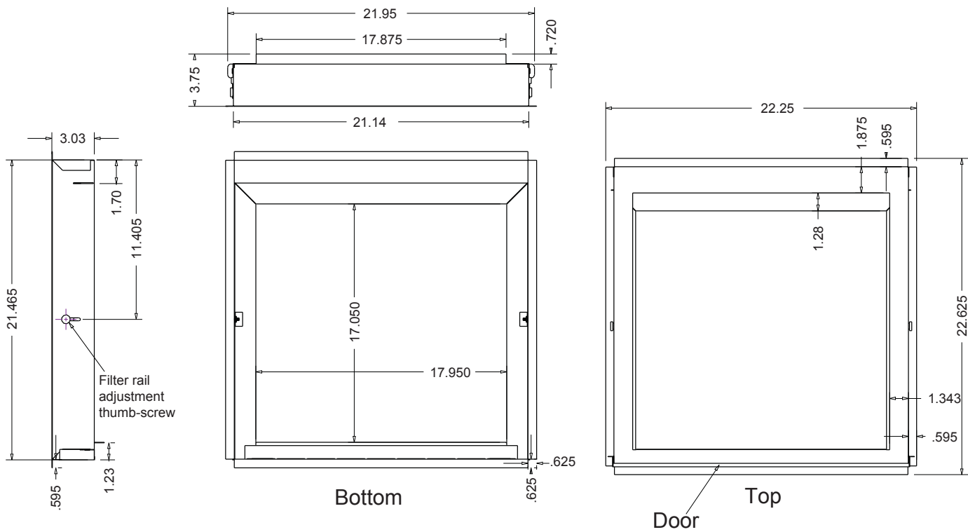
V1FBS02-4P Dimensions (inches)
