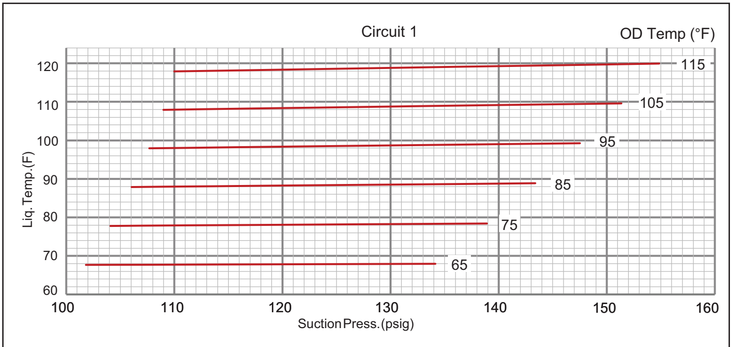
LGT/LCT 300 NO REHEAT CHARGING CURVE CIRCUIT 1 - ALL-ALUMINUM OD COIL - 581098-02
