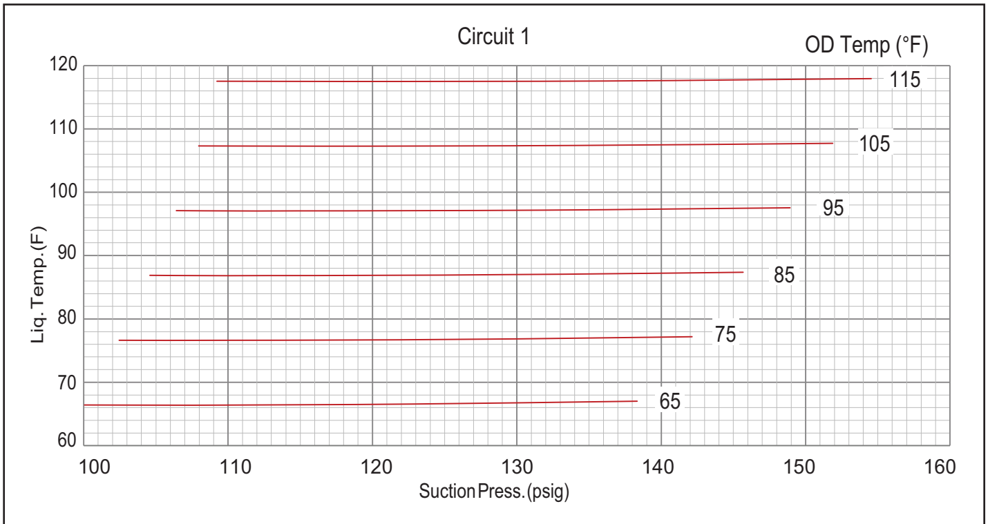
LGT/LCT 240 NO REHEAT CHARGING CURVE CIRCUIT 1 - ALL-ALUMINUM OD COIL - 581094-02
