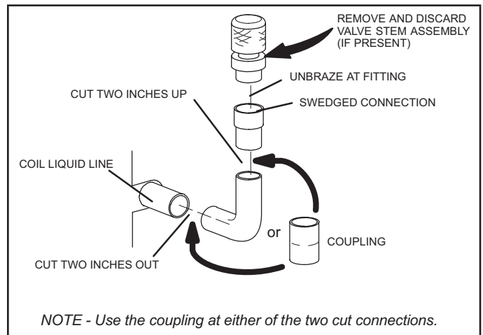
FIGURE 3. CK40CT Liquid Line Connections
