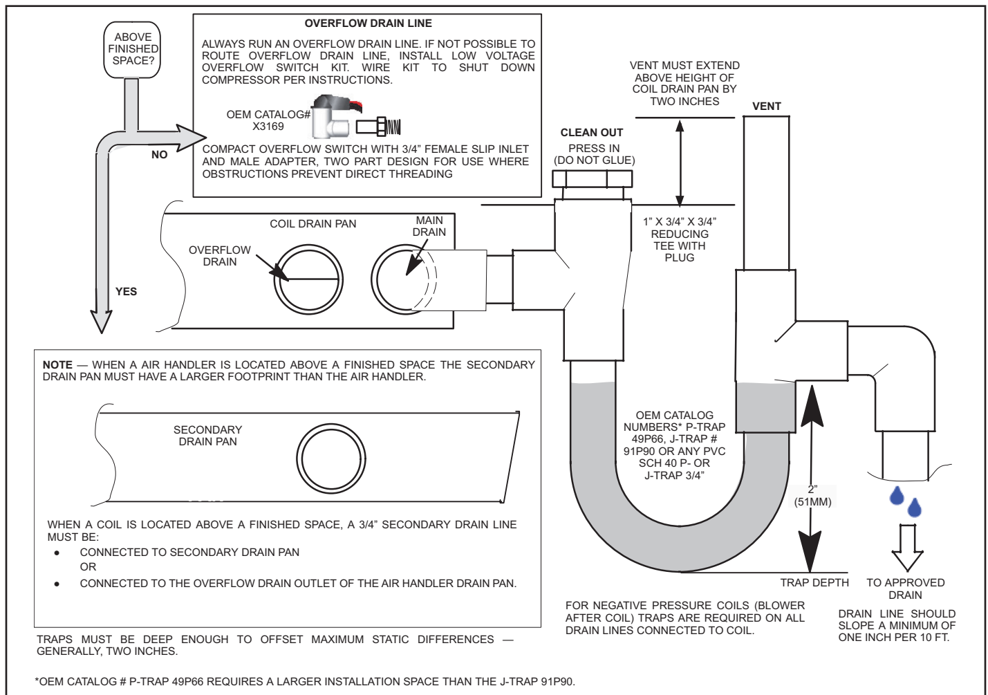
FIGURE 4. Typical Main and Overflow Drain Installations
