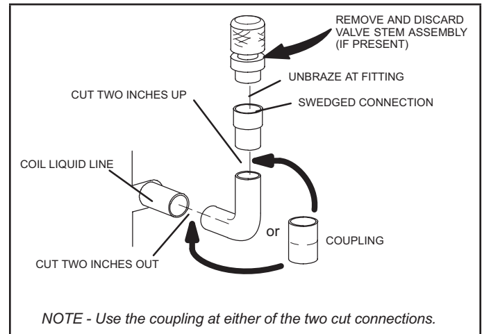
FIGURE 2. CK40DT Liquid Line Connections
