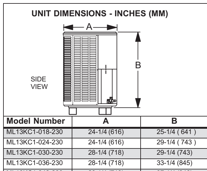
FIGURE 1. Unit Dimensions
