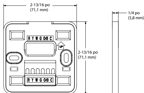
Figure 1. Thermostat intelligent L40 de Lennox, couvercle et plaque murale
