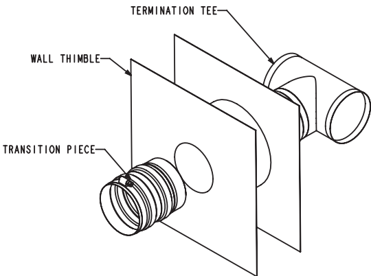
HORIZONTAL VENT KITS (DOWNSLOPE)
