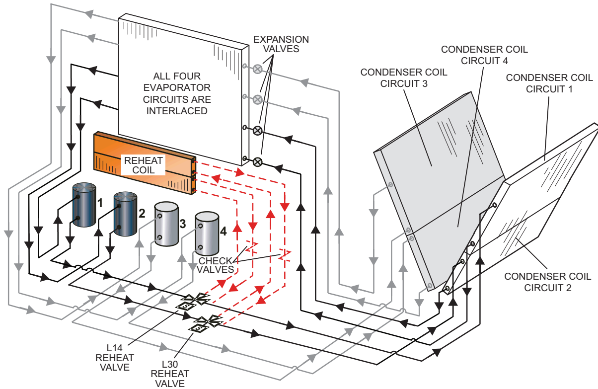
REFRIGERANT SCHEMATIC (210, 240 and 300 MODELS ONLY)
