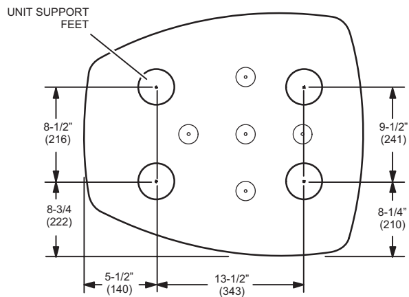
EL15KC1-018 & EL15KC1-024 BASE SECTION (SMALL)
