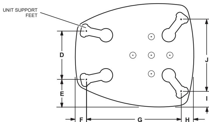
EL15KC1-030 TO -060 BASE WITH ELONGATED LEGS
