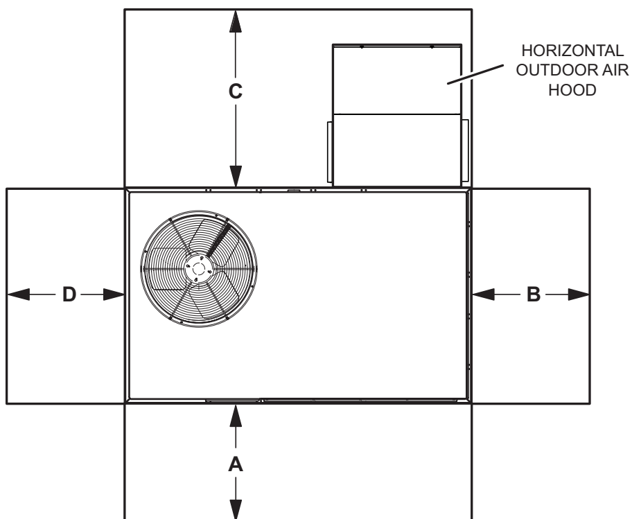
UNIT WITH HORIZONTAL ECONOMIZER
