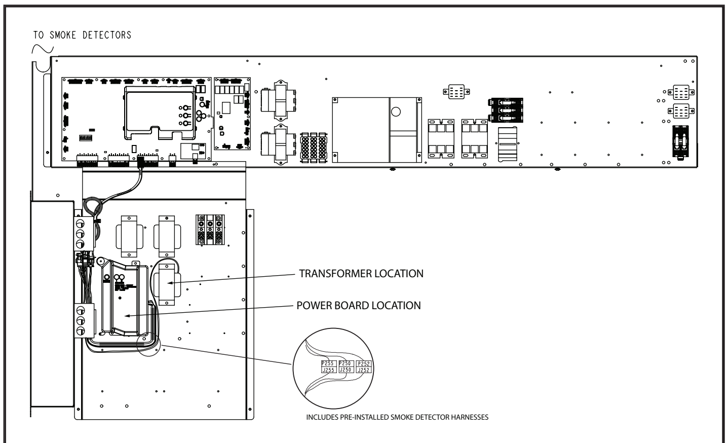
FIGURE 12 Power Board / Transformer Locations On M4 Boards (D-Box)
