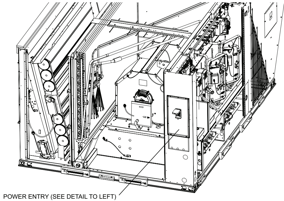
FIGURE 7 Transformer Harness Routing - SH/SD
