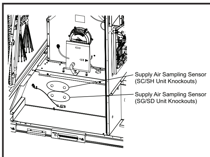
FIGURE 3 Knockouts for Smoke Detector Sensor
