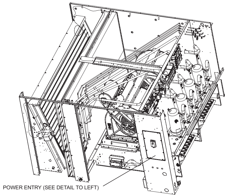
FIGURE 5 Transformer Harness Routing
