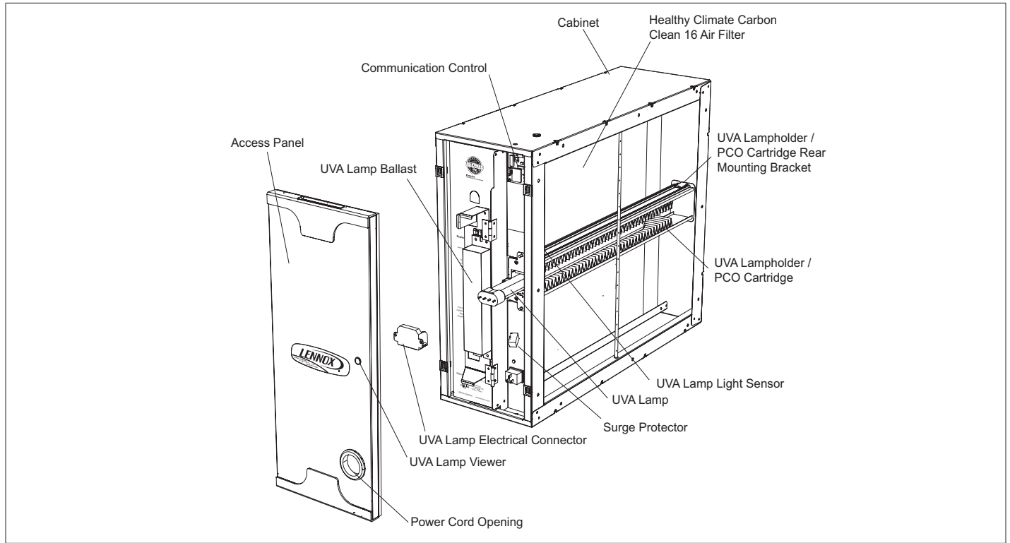
Figure 1. Parts Identification
