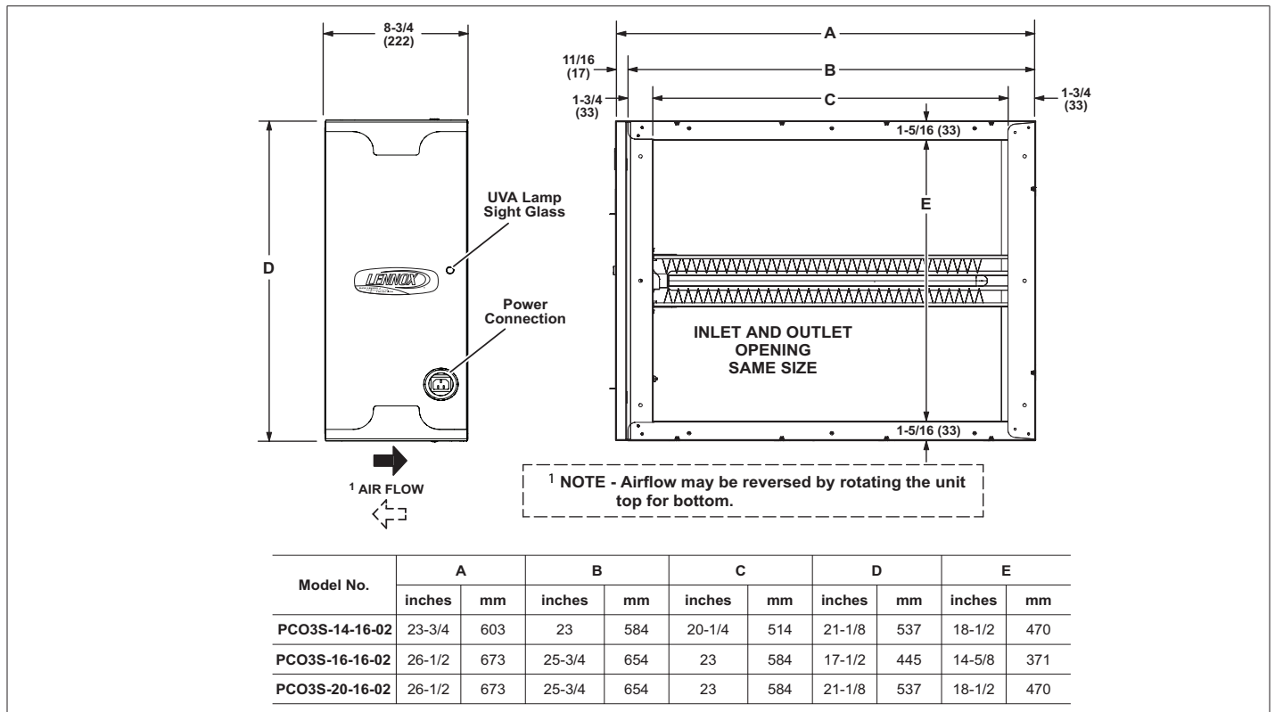
Figure 2. Dimensions
