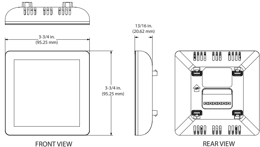
Figure 2. Thermostat Dimensions
